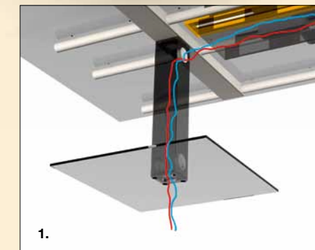
1. Column base with hole for cable passage.
